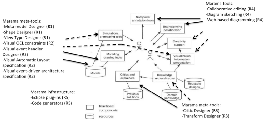
Figure 3. Relating Sutcliffe's model to Marama capabilities.
