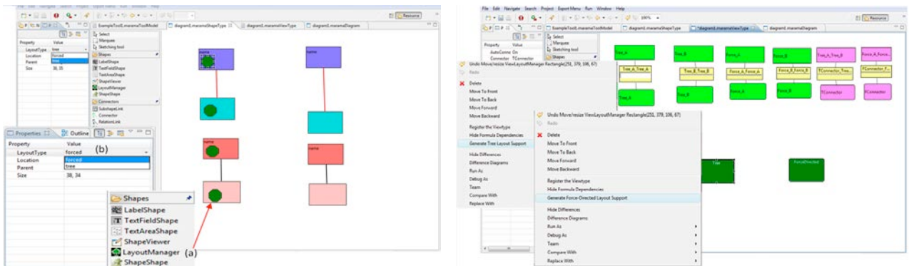
Figure 9. Specifying participation in auto-layouts (left) and type of auto-layout(s) to add to a view type definition (right).
