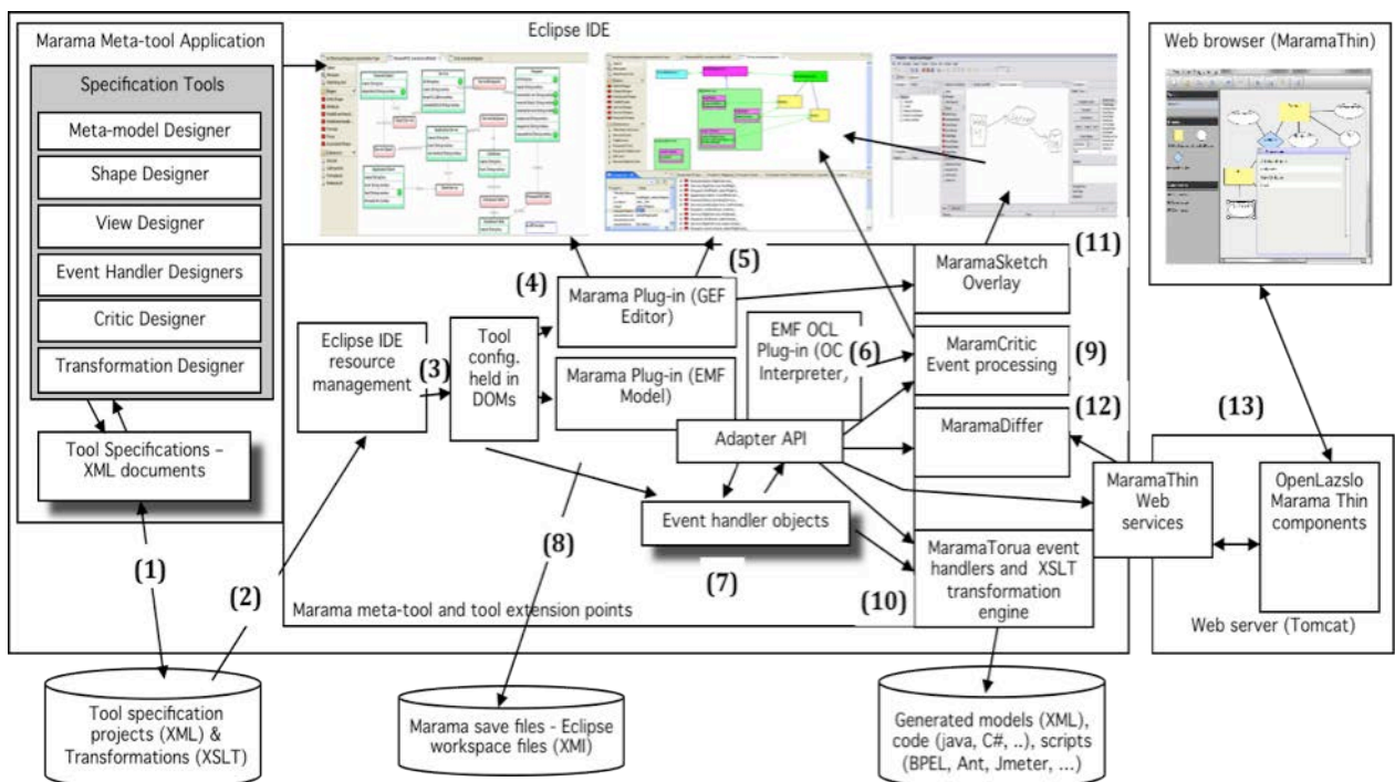
Figure 17. The basic architecture of Marama.
