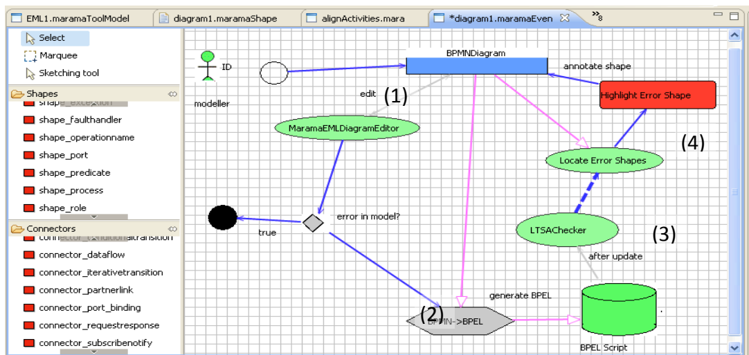
Figure 12. Event-based tool architecture integration specification.
