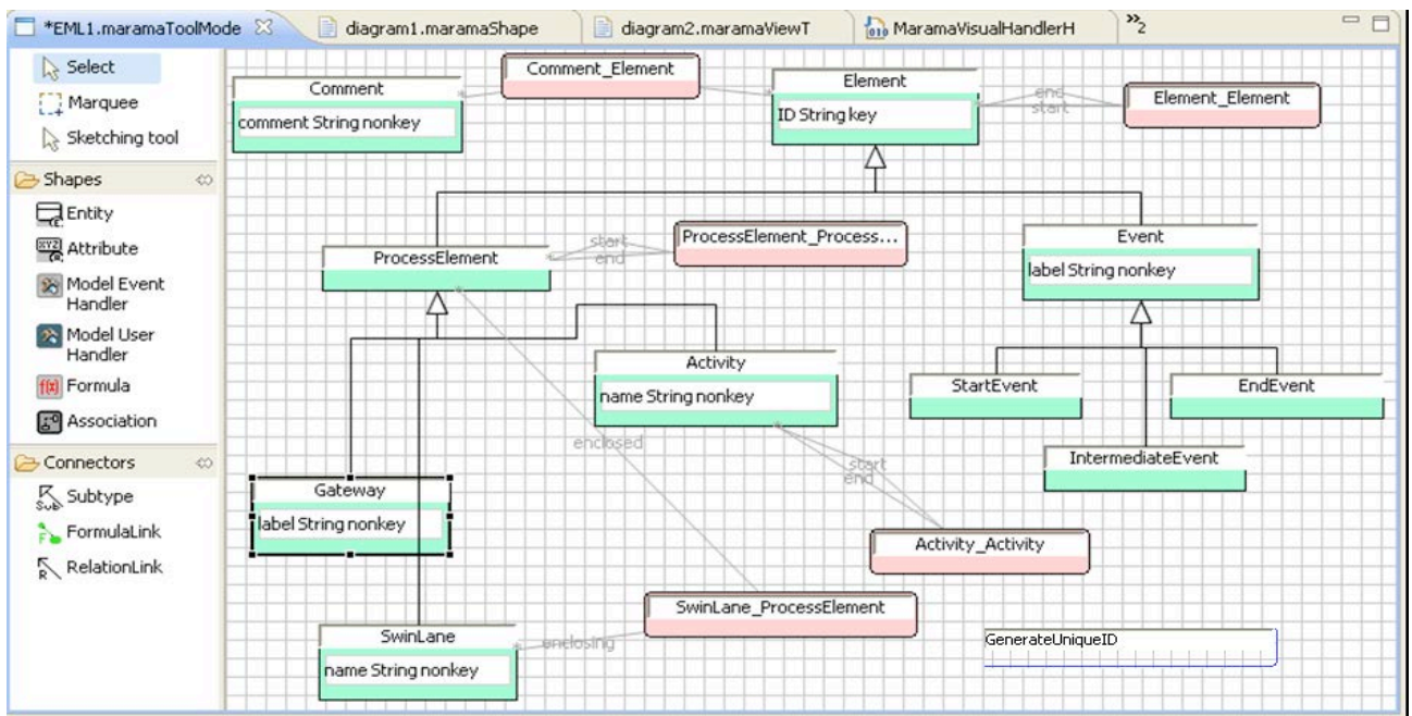
Figure 4. An example MaramaEML meta-model in the Marama meta-model designer tool.
