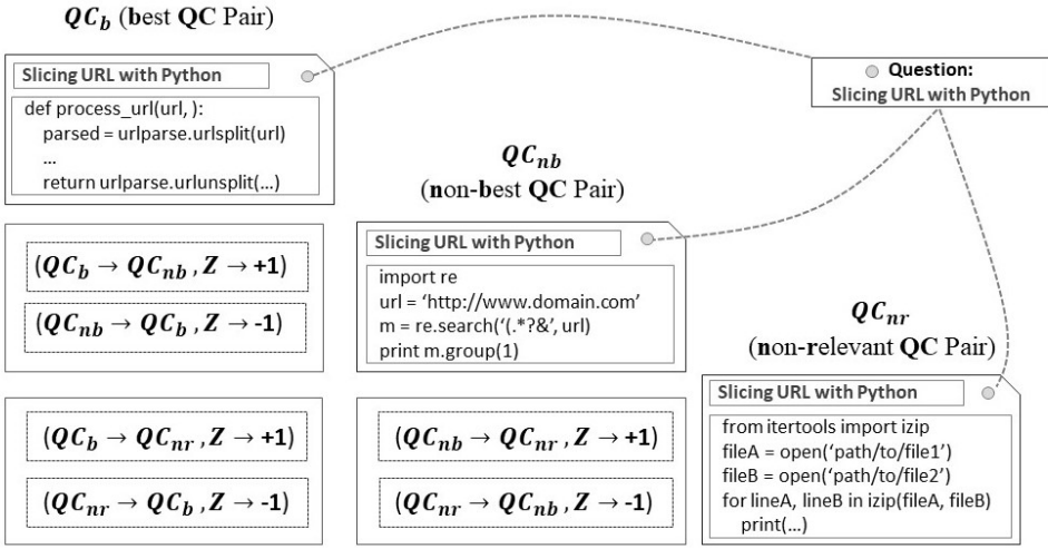
Fig. 5. Preference-Pairs Construction
