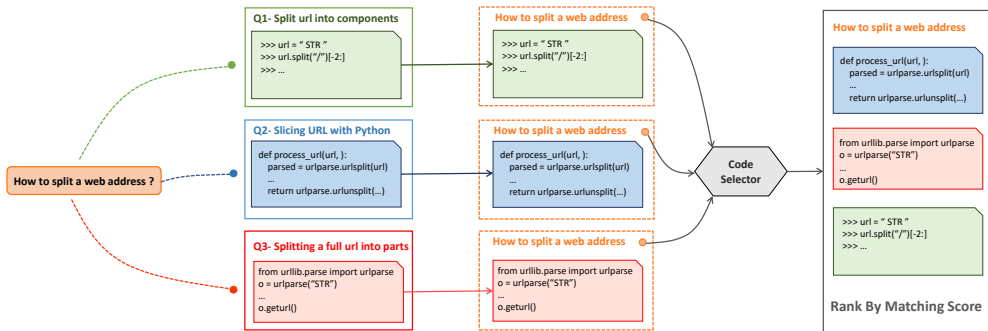
Fig. 4. CodeSelector Workflow
