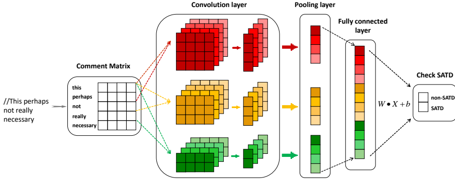
Fig. 2. Convolutional Neural Network Architecture (4 filters for each filter size ( h = 2, 3, \text{ or } 4 ))
