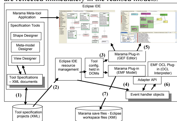
Figure 1: Marama architecture
