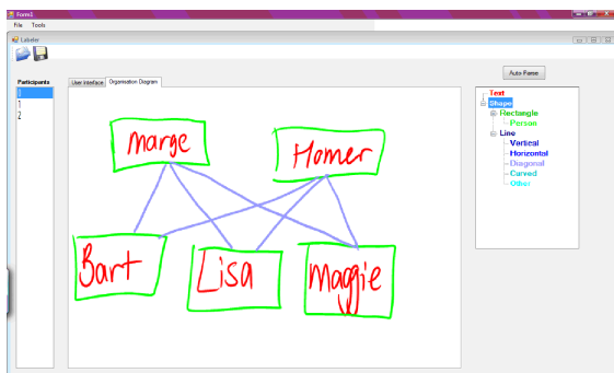
Figure 6: Labeller form showing a diagram labelled manually.
