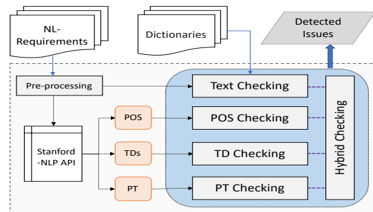
Fig. 1: NL-Requirements Quality Checking Tool
