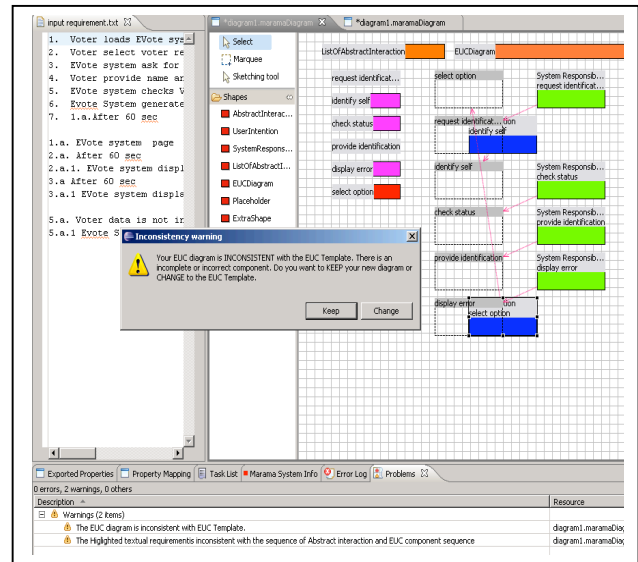
Figure 3. Visual Differencing for completeness and correctness checking
