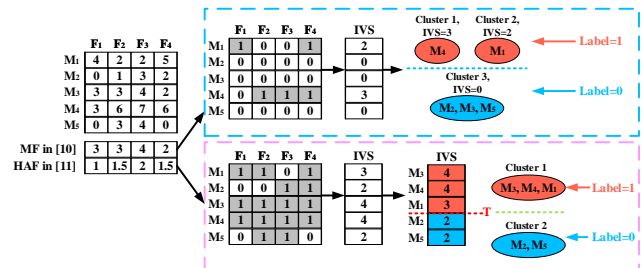
Figure 2: The process of labeling scheme 4 and 5.
