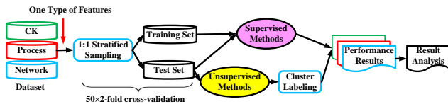
Figure 4: Framework of our empirical study.
