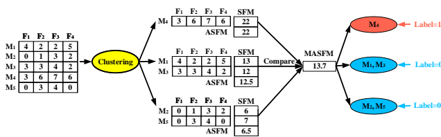
Figure 5: Labeling scheme for multiple clusters.
