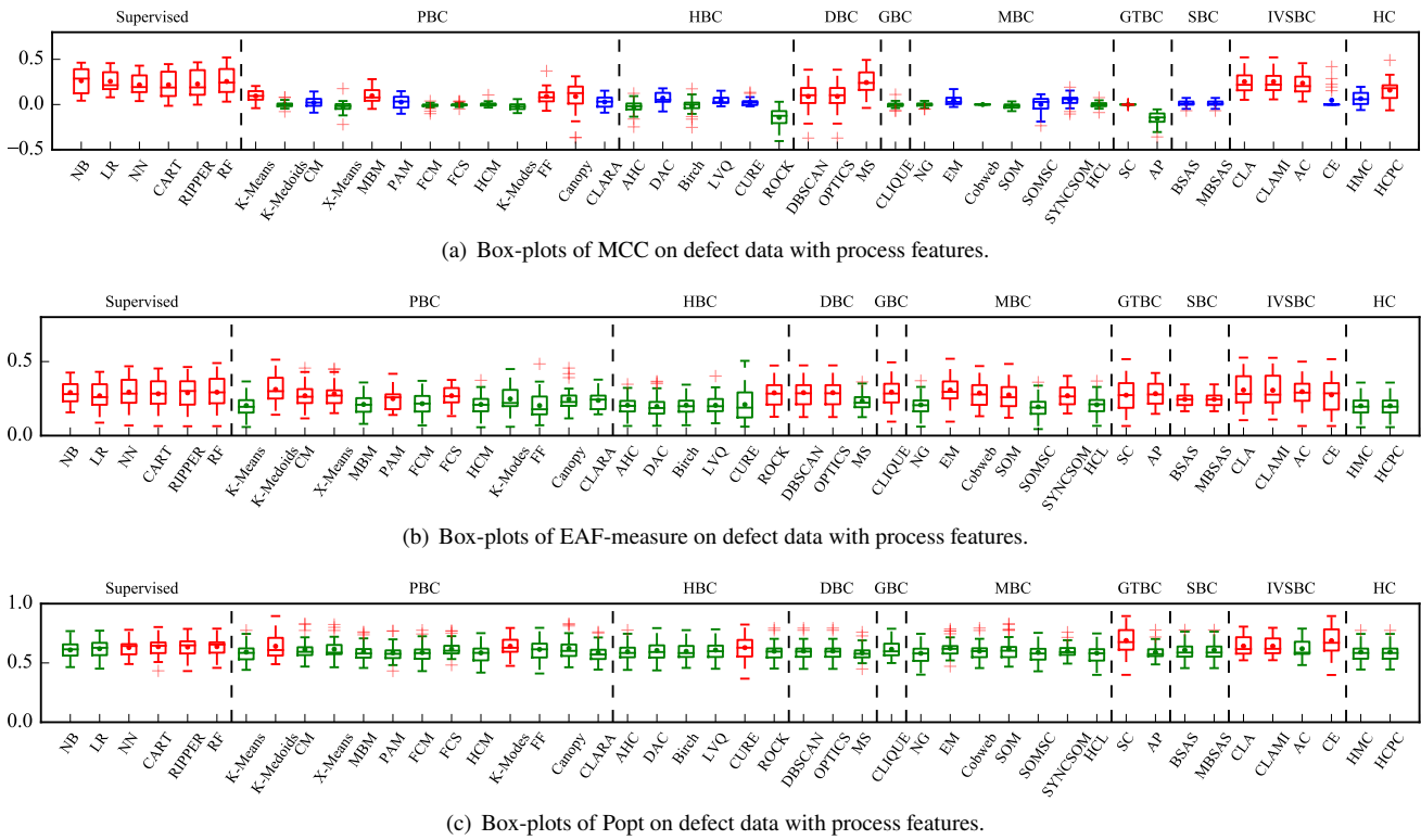
Figure 9: Box-plots of 3 indicator values across 27 defect data with process features.
