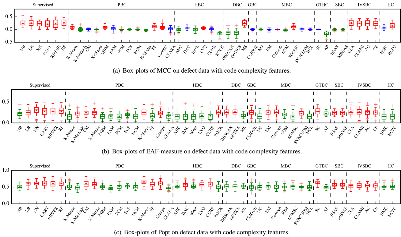
Figure 8: Box-plots of the 3 indicator values across 27 defect data with code complexity features.
