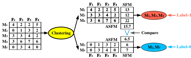
Figure 3: The process of labeling scheme 6.
