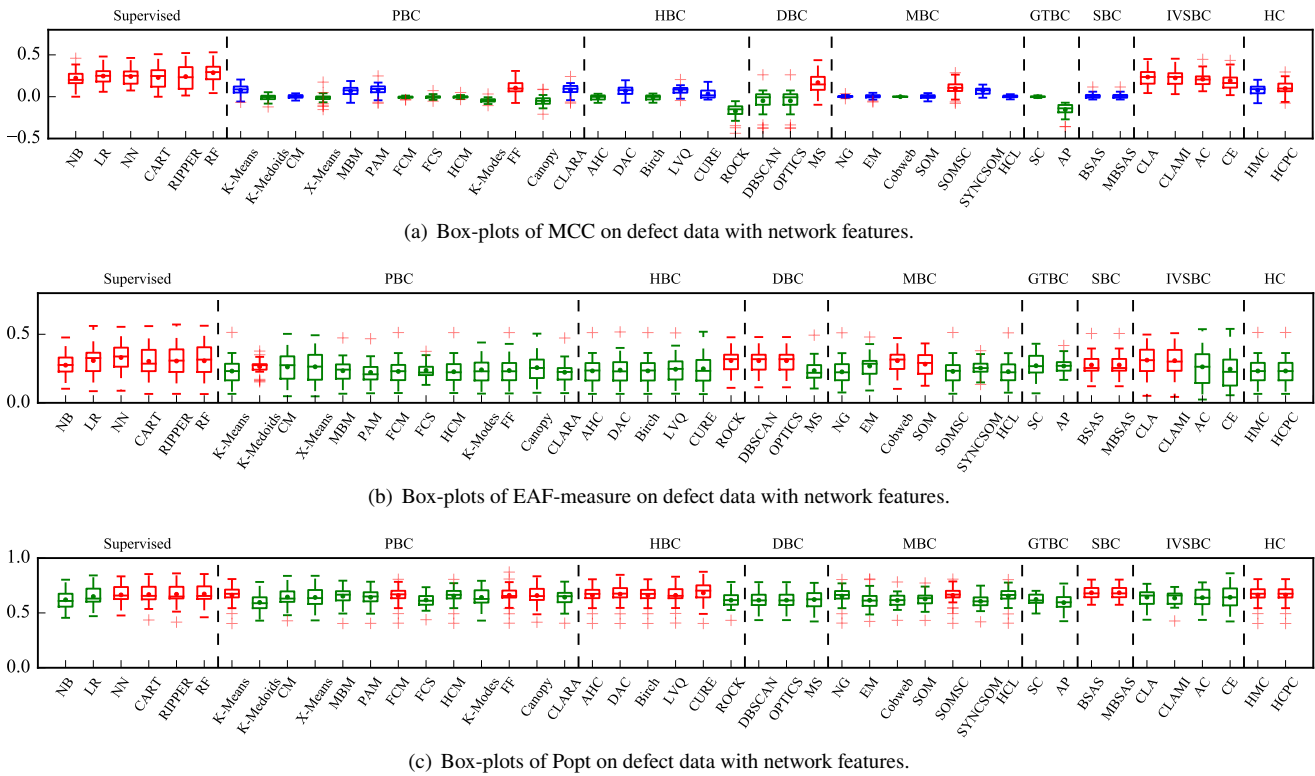
Figure 10: Box-plots of 3 indicator values across 27 defect data with network features.
