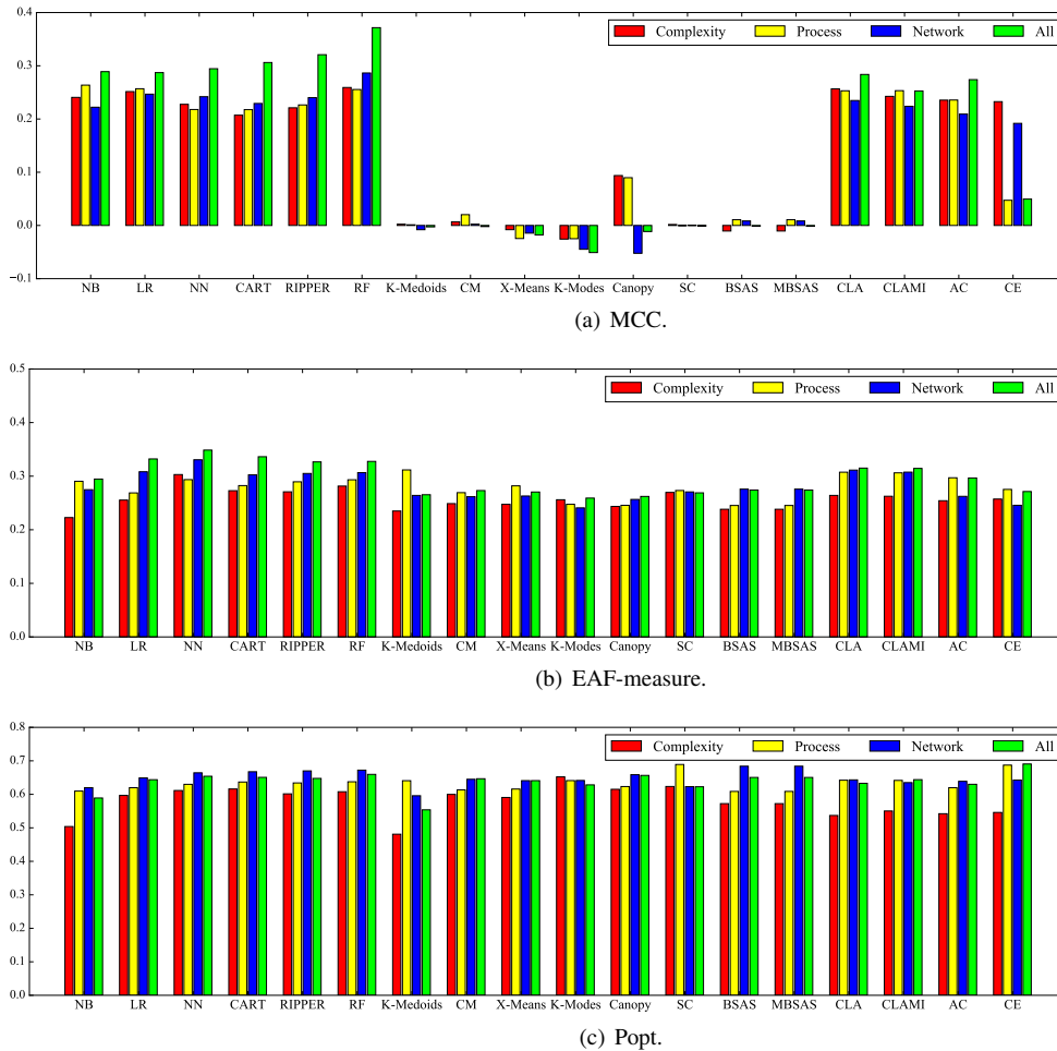
Figure 12: Average values of 3 indicator for the selected methods on defect data with different feature types and the combined features.
