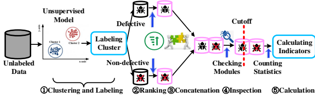
Figure 6: Calculation process for effort aware indicators.
