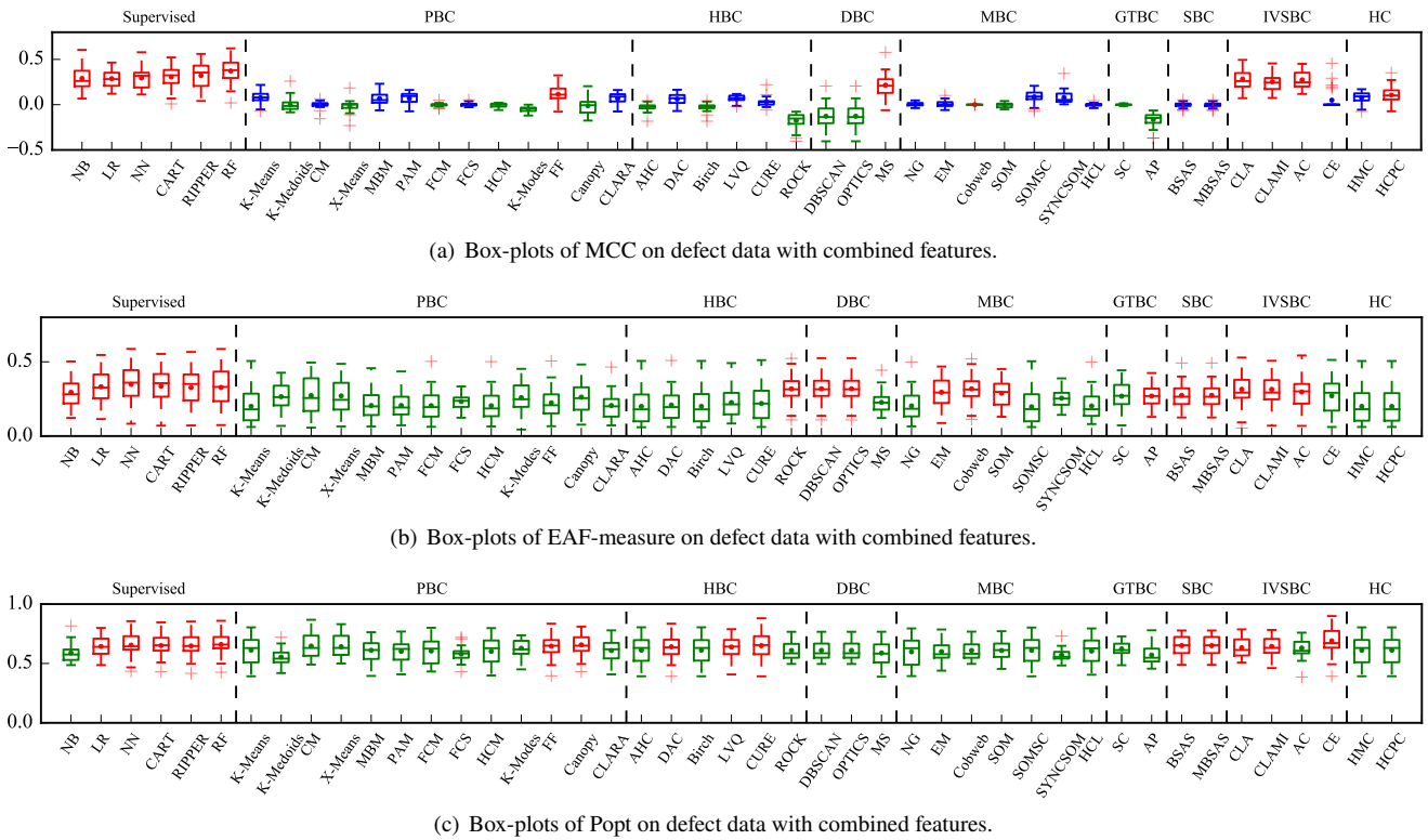
Figure 11: Box-plots of 3 indicator values across 27 defect data by combining the 3 types of features.
