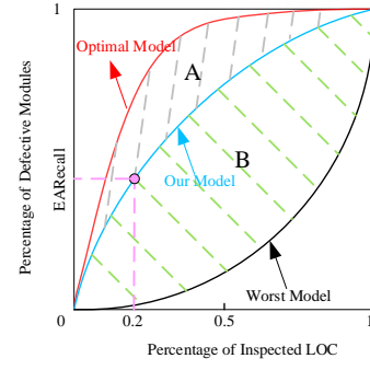
Figure 7: LOC-based Alberg diagram
