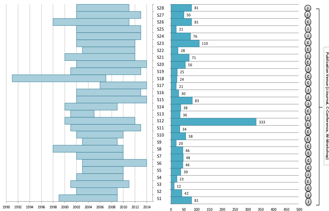
Fig. 5a: Years covered by primary studies of the SLRs
