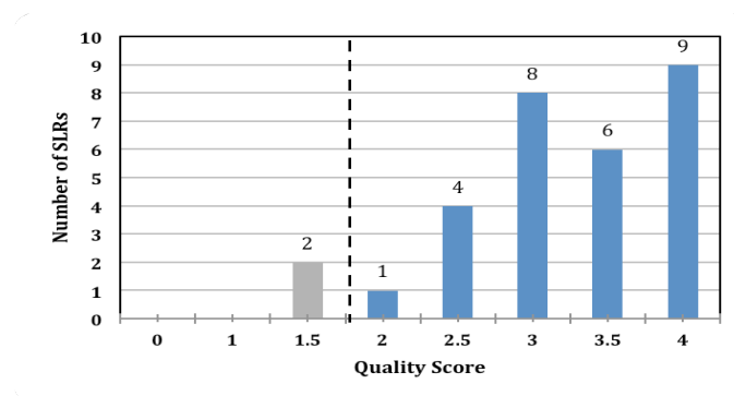
Fig. 2. Quality scores of SLRs (2 excluded studies shown before cut-off line)
