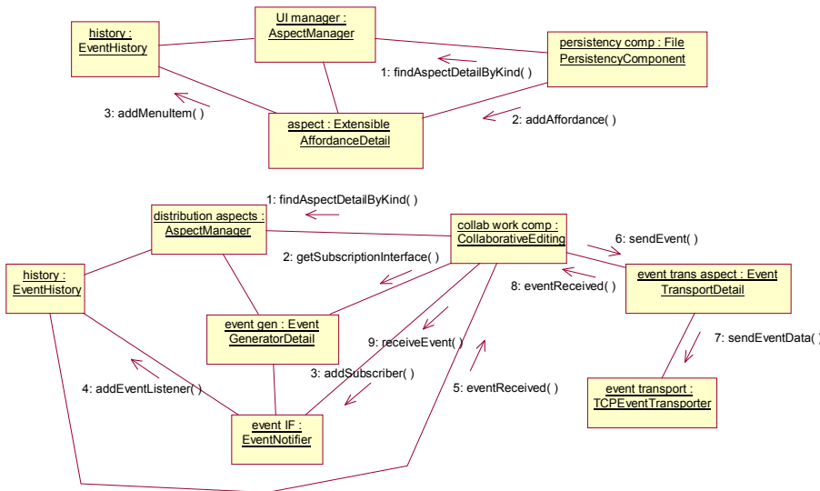
Fig. 8. (a) User interface extension; and (b) event subscription service access via AspectDetail objects.
