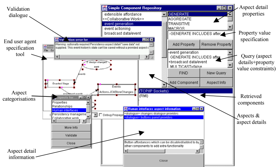
Fig. 9. End user access to aspect information (left) and component retrieval using aspects (right).
