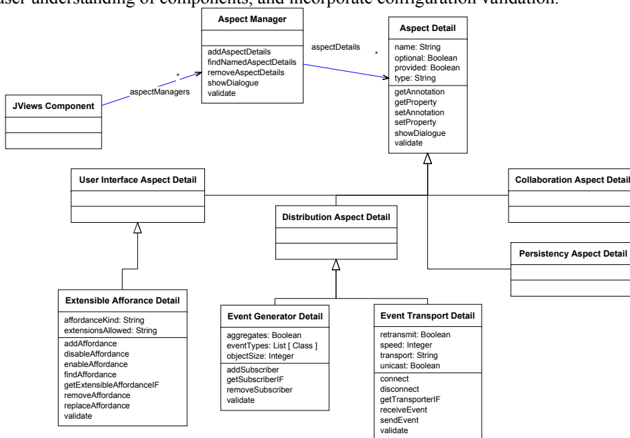
Fig. 7. Some AspectManager and AspectDetail classes from the JViews framework.
