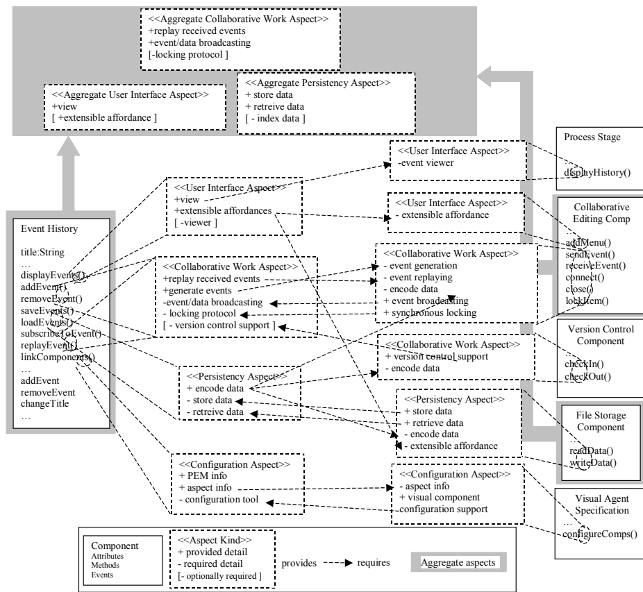
Fig. 4. Visual representation of Serendipity-II components and some of their requirements-level aspects.
