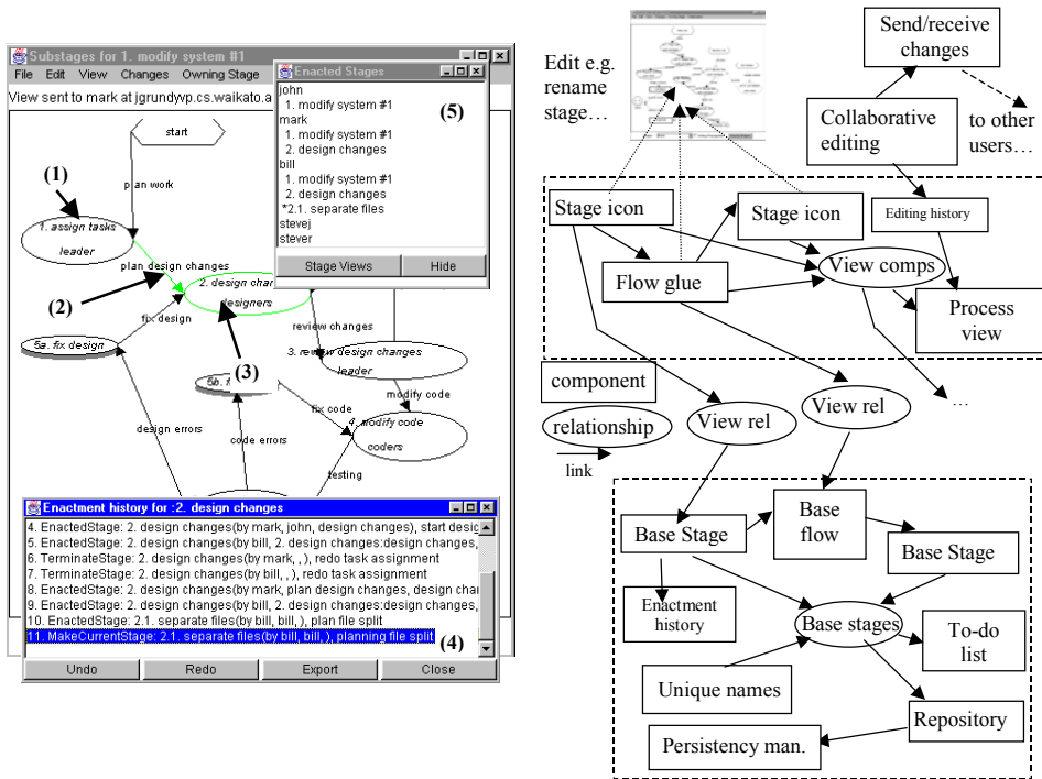
Fig 1. (a) Serendipity-II process management tool; and (b) example components.
