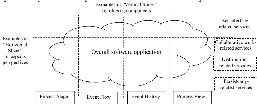
Fig. 2. General concepts of components vs. component aspects.
