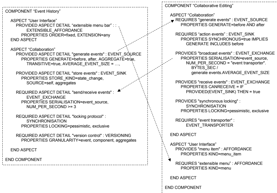
Fig. 5. Textual codification of some Serendipity-II aspect detail properties.
