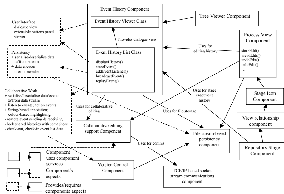
Fig. 6. Some design-level components and aspects for Serendipity-II.
