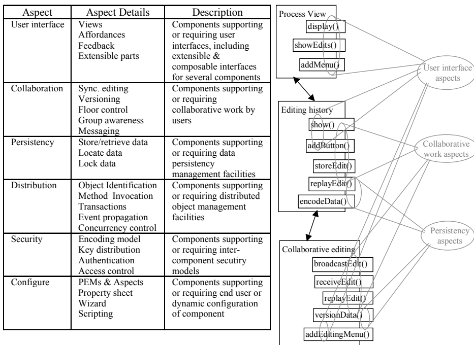
Fig. 3. (a) Some general aspects; and (b) an illustration of component aspects from Serendipity-II.
