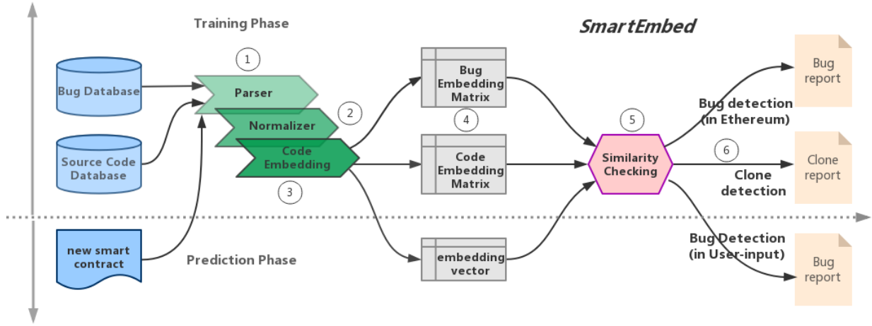
Fig. 1. Overview of Our Approach
