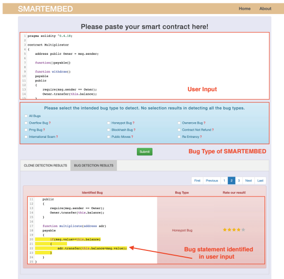
Fig. 3. Sample Results of Bug Detection
