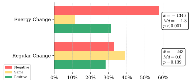
Fig. 5. Maintainability differences for energy commits and baseline commits. In the case of the regular commits, used as a baseline, 33.0% decrease maintainability (183 cases), 38.7% do not change maintainability (215 cases), and 28.3% improve maintainability (157 cases). Since the p-value of the Wilcoxon signed-rank test ( p = 0.139 ) is not below the significance level ( \alpha = 0.05 ), there is no statistical significance of the impact of regular commits on maintainability.
