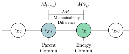
Fig. 3. Maintainability difference for the energy commit v_E .
