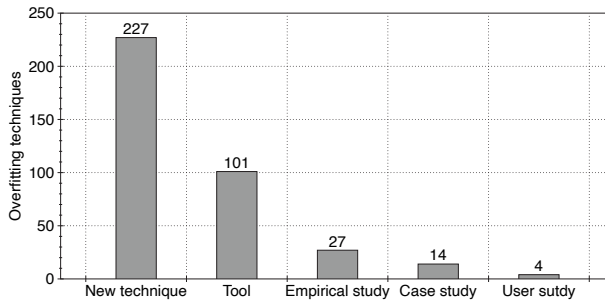
Fig. 7. Types of main contributions
