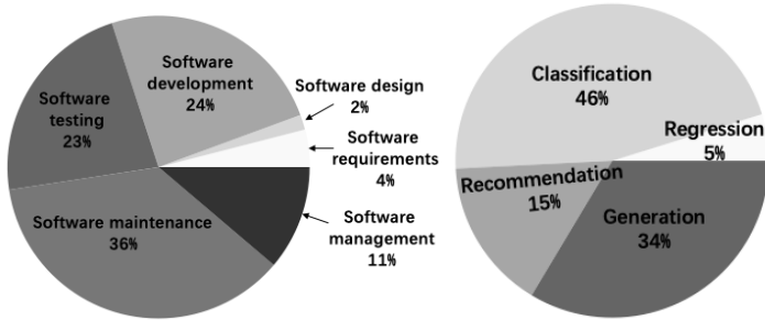
Fig. 2. The distribution of DL tech-techniques in Different SE activities. Fig. 3. The classification of primary studies.
