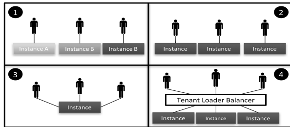
Figure 2: Multi-tenancy approaches [13]
