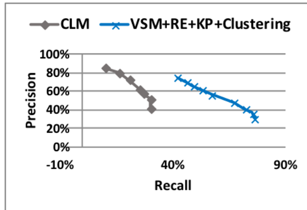
(c) EasyClinic: CLM (CC-TC(ID)) vs Our Approach (CC-TC)
